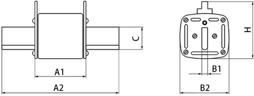
NT1/NT2/NT3尺寸图 NT1/NT2/NT3Dimension drawing
