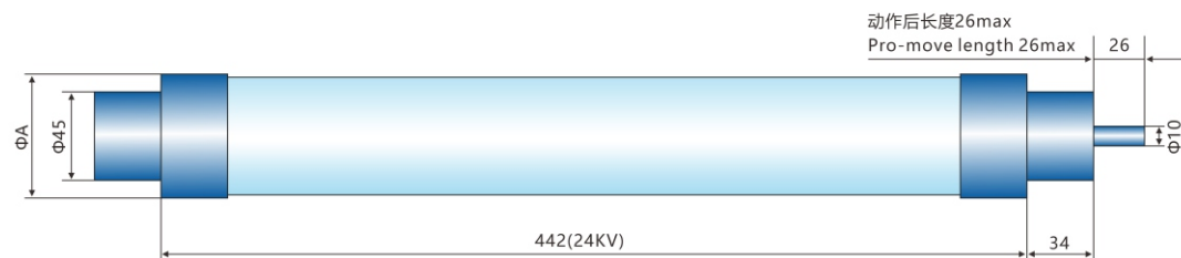
熔断器Char1/a link XRNT□-24KV
