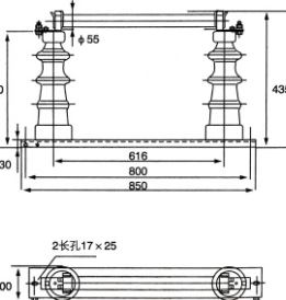
RN2-35/0.5型外形尺寸 RN2-35/0.5 External dimensions of the type
