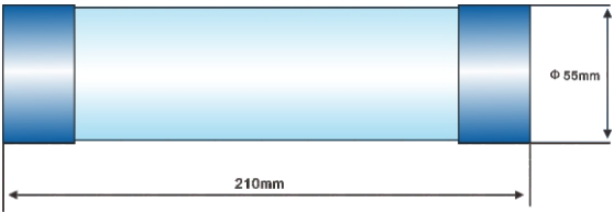
RN2-6KV/10KV尺寸图 (Dimension drawing)
