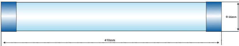
RN1-10KV尺寸图 (Dimension drawing)
