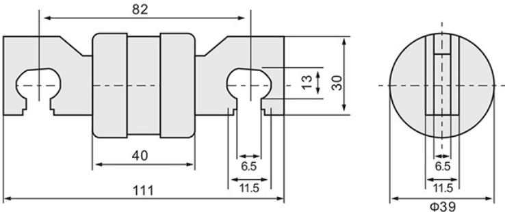
RGS88尺寸图 Dimension drawing
