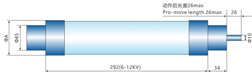
熔断器Char1/a link XRNT□-12KV
