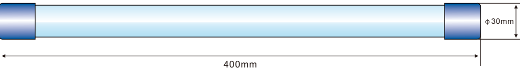
XRNP1-40.5KV尺寸图 (Dimension drawing)
