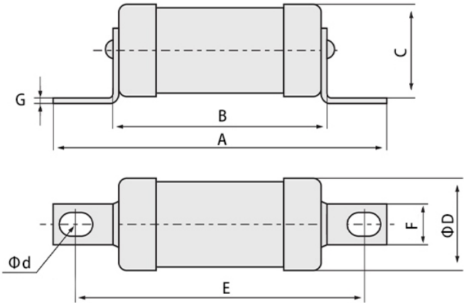
其它型号尺寸图 Dimension diagrams of other models
