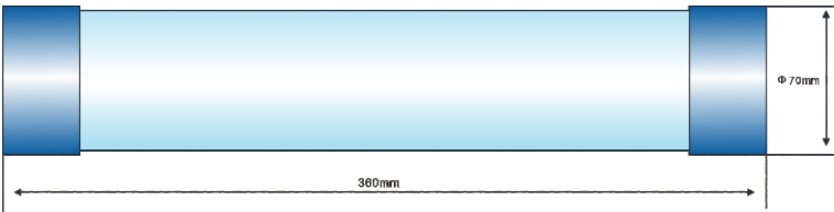
RN1/RN3-10KV尺寸图 (Dimension drawing)
