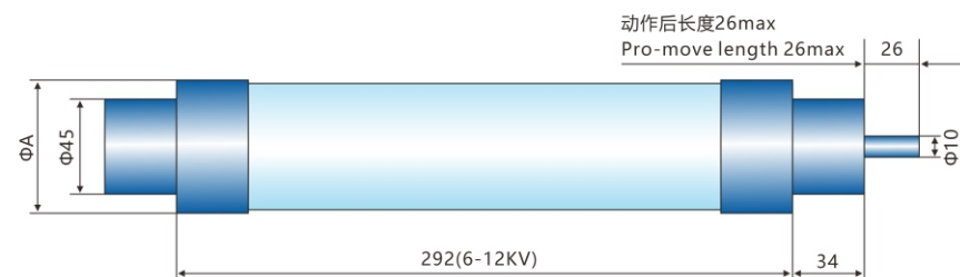
熔断器Char1/a link XRNT□-12KV
