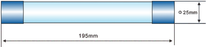
XRNP1-24KV尺寸图 (Dimension drawing)
