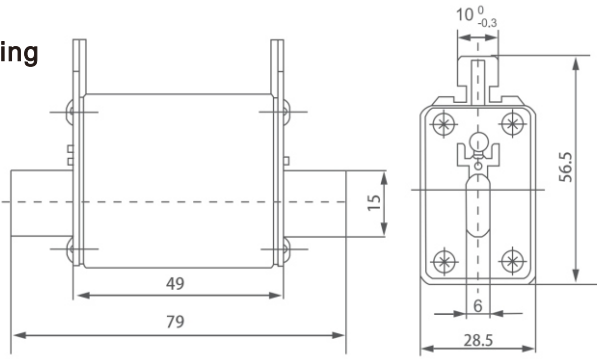
NT1/NT2/NT3尺寸图 NT1/NT2/NT3Dimension drawing
